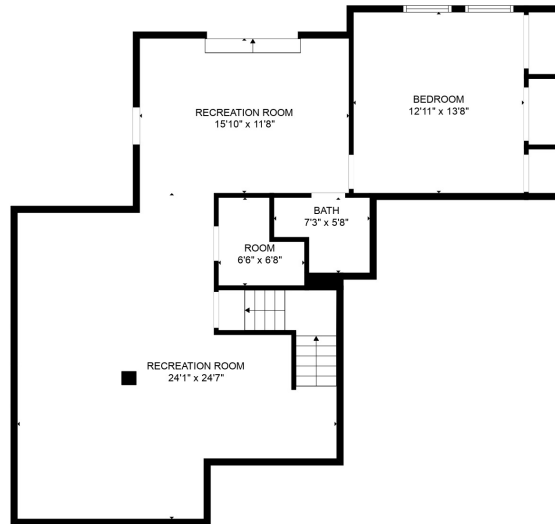
FLOOR 2
